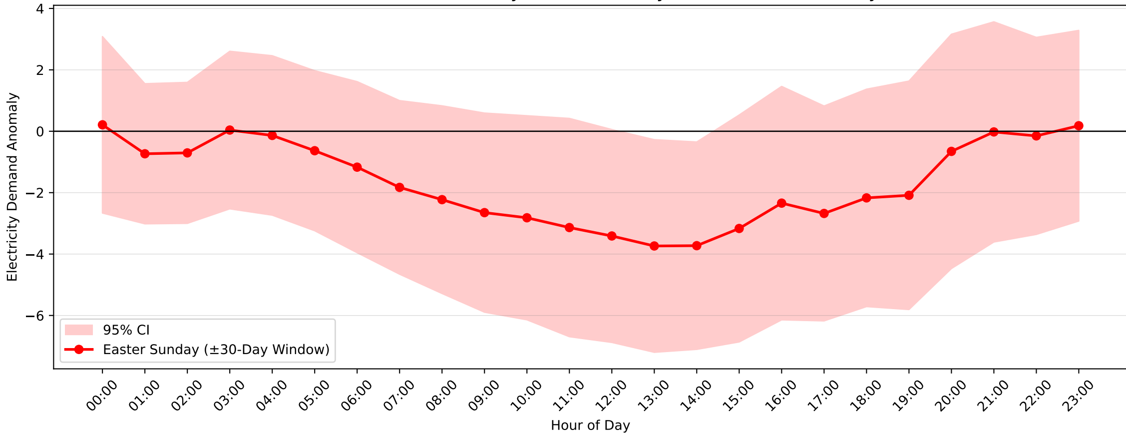
Broadmeadow Demand Anomaly: Easter Sunday (2004–2017, \pm 30 -Day Window)
